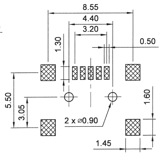
RECOMMENDED P.C.B PATTERN LAYOUT
